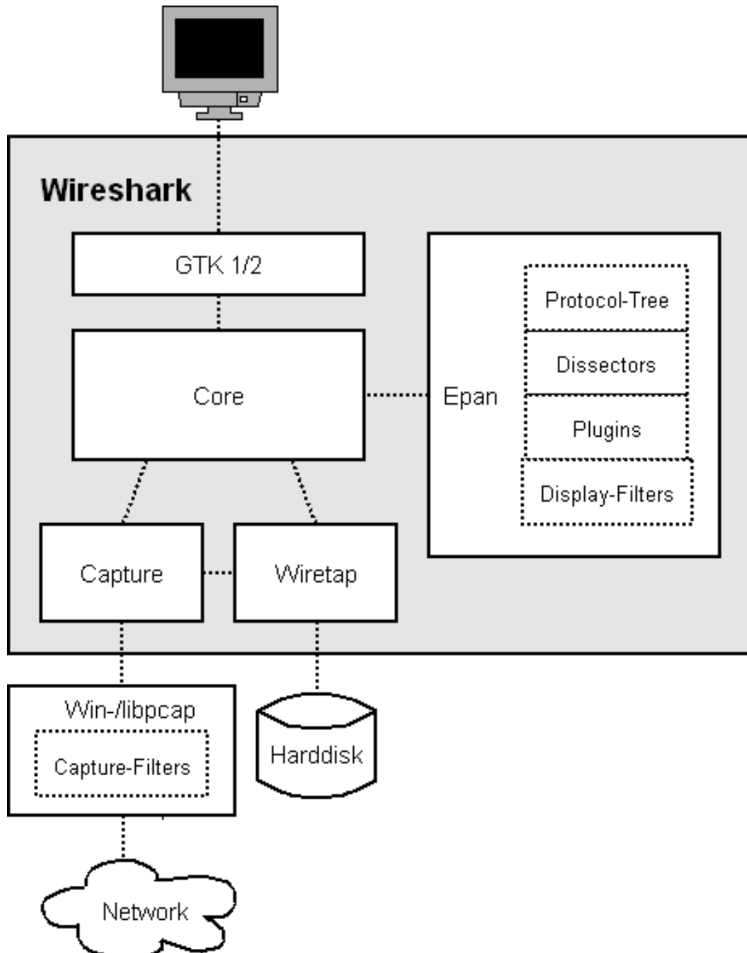
Figure 6.1. Wireshark function blocks.
